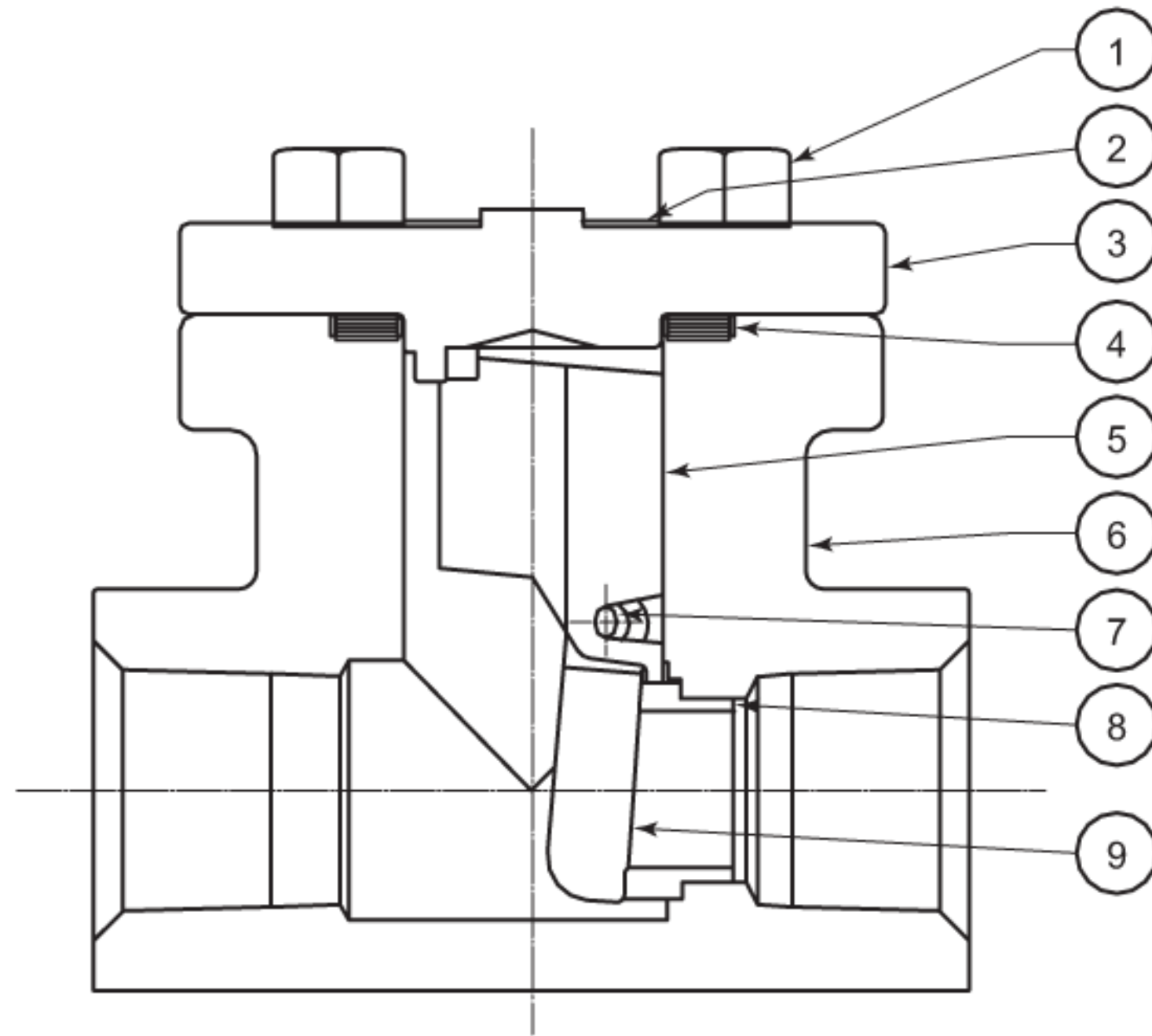
Figure E.9—Swing Check Valve
