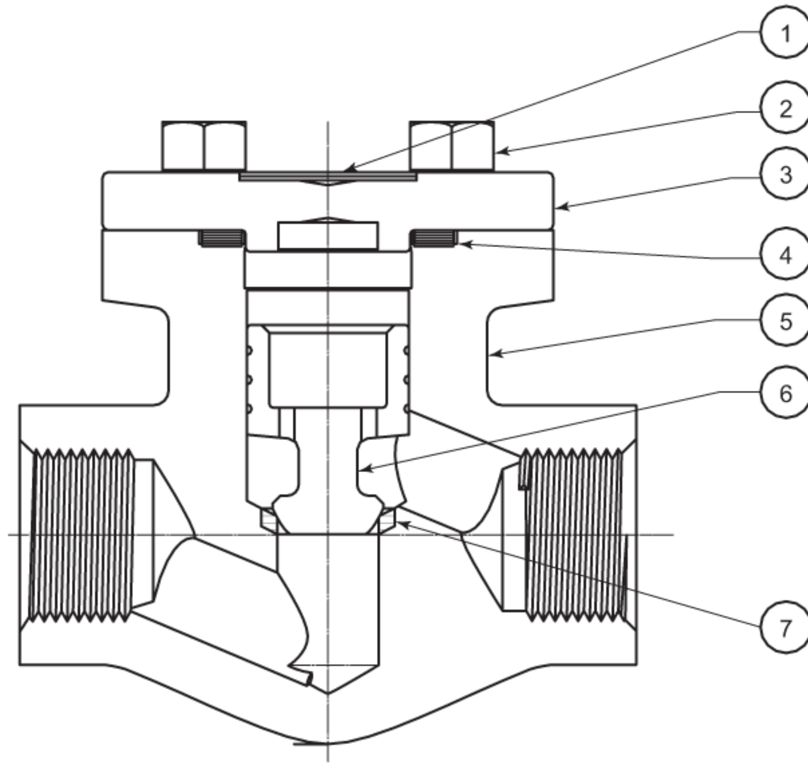
Figure E.7—Piston Check Valve
