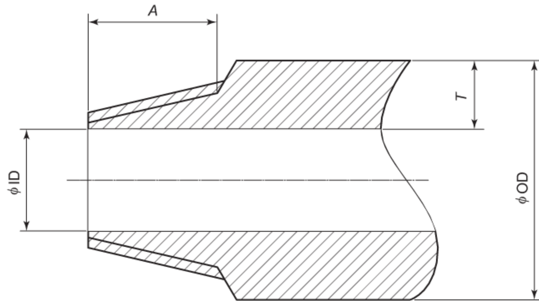
Figure B.1—Threaded End Extension for Class 800
