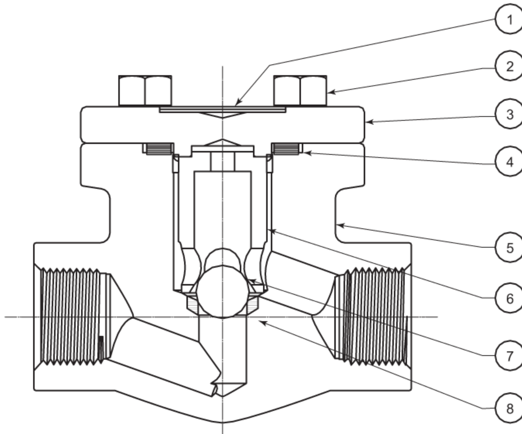
Figure E.8—Ball Check Valve
