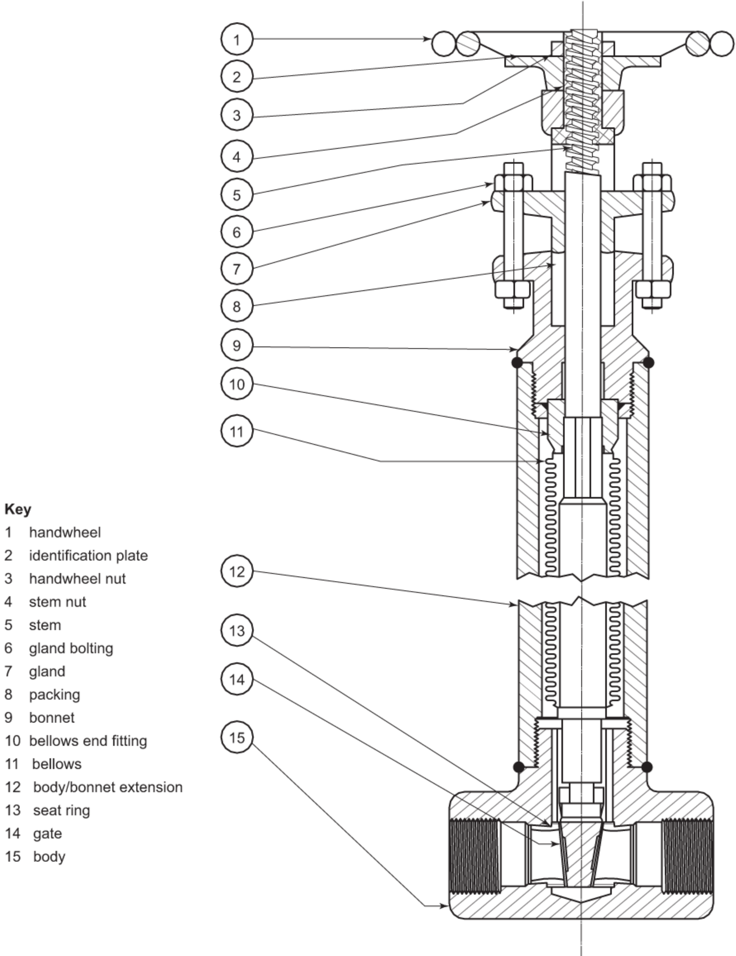
Figure E.3—Bellows Stem Seal Gate Valve
