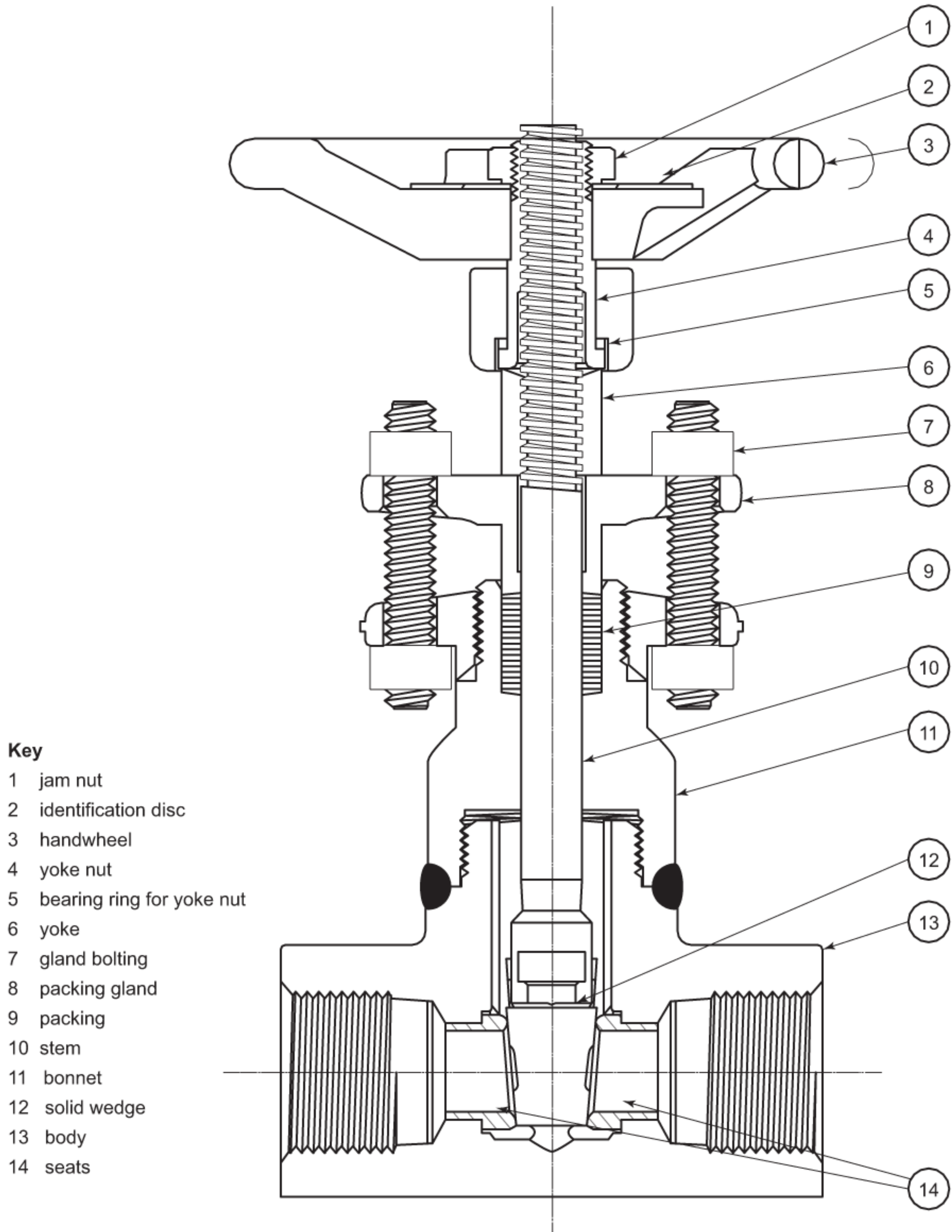
Figure E.4—Welded Bonnet Gate Valve
