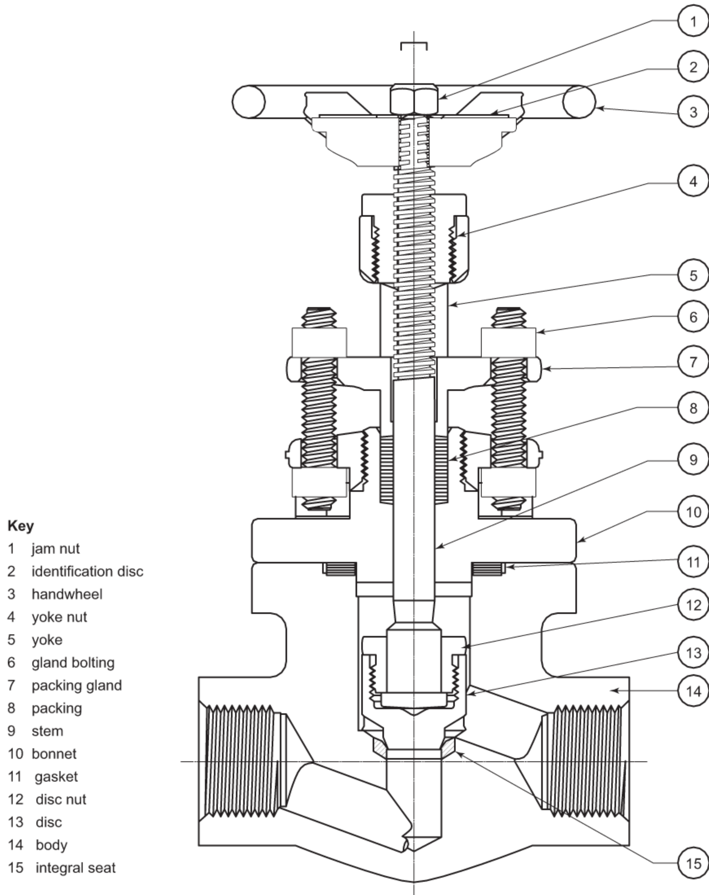
Figure E.5—Outside Screw and Yoke Globe Valve
