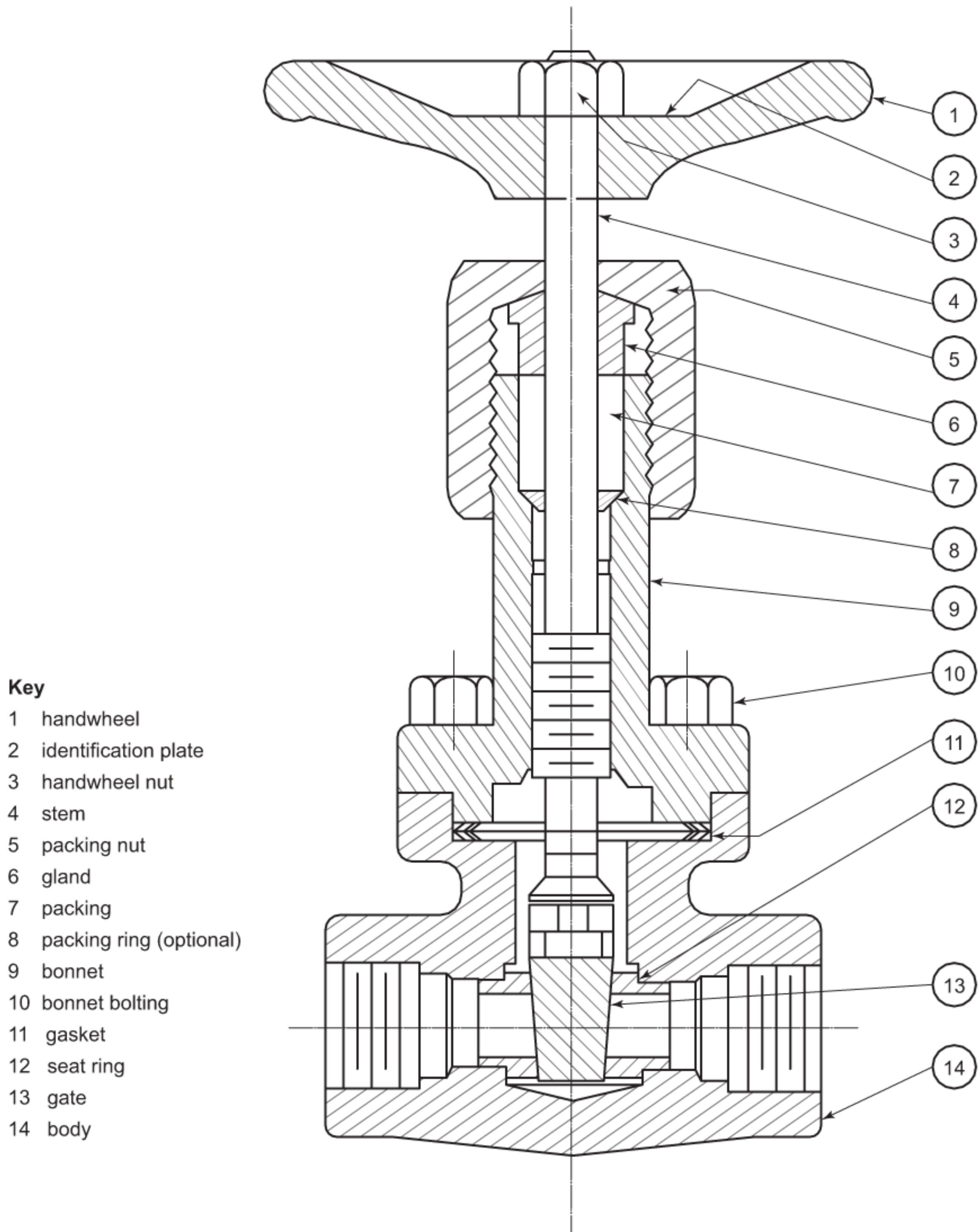
Figure E.2—Inside Screw Gate Valve
