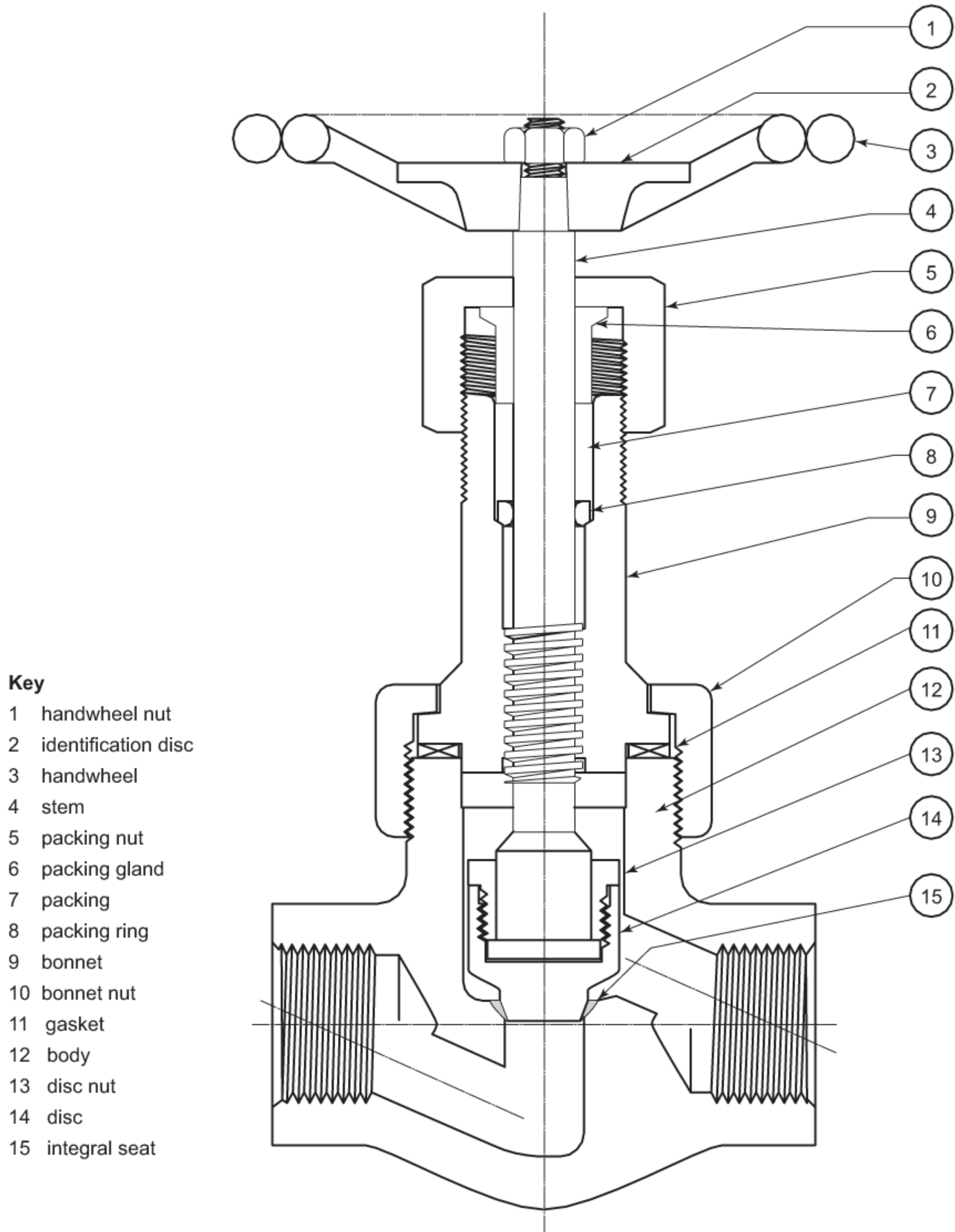
Figure E.6—Union Bonnet Globe Valve
