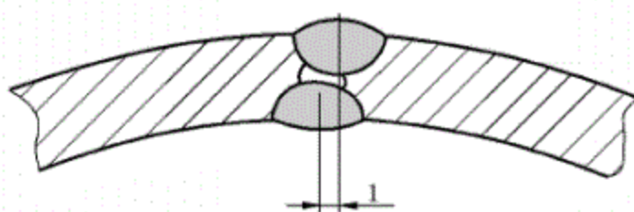
d) SAW 管焊道焊偏
